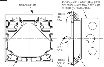
ATTACH MOUNTING PLATE TO PLASTER RING USING FOUR (4) SCREWS (SUPPLIED)
